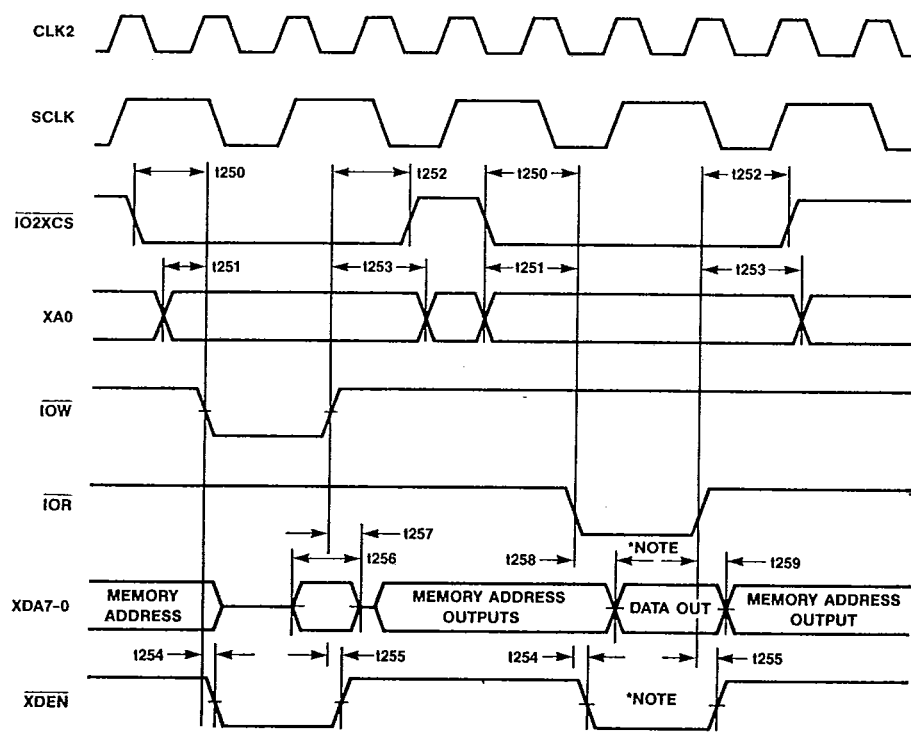
32C302 TIMING DIAGRAM (IO READ/WRITE)
