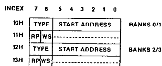
Figure 2.6. DRAM Configuration/Timing Register Summary
