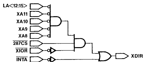
82A304 TTL Equivalent Chip Select Generation Circuitry
