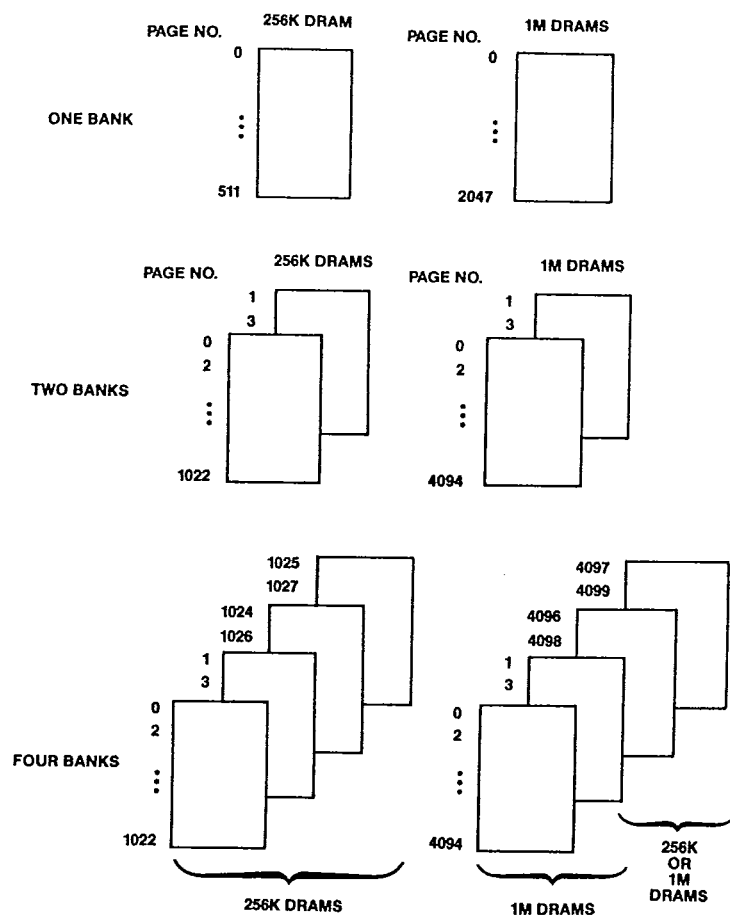
Figure 2-2. Memory Addressing
