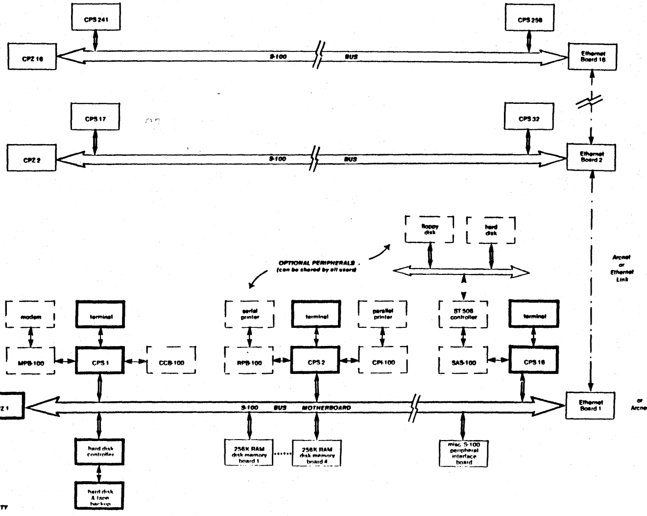
TURBODOS MASTER/SLAVE WORK ARCHITECTURE
